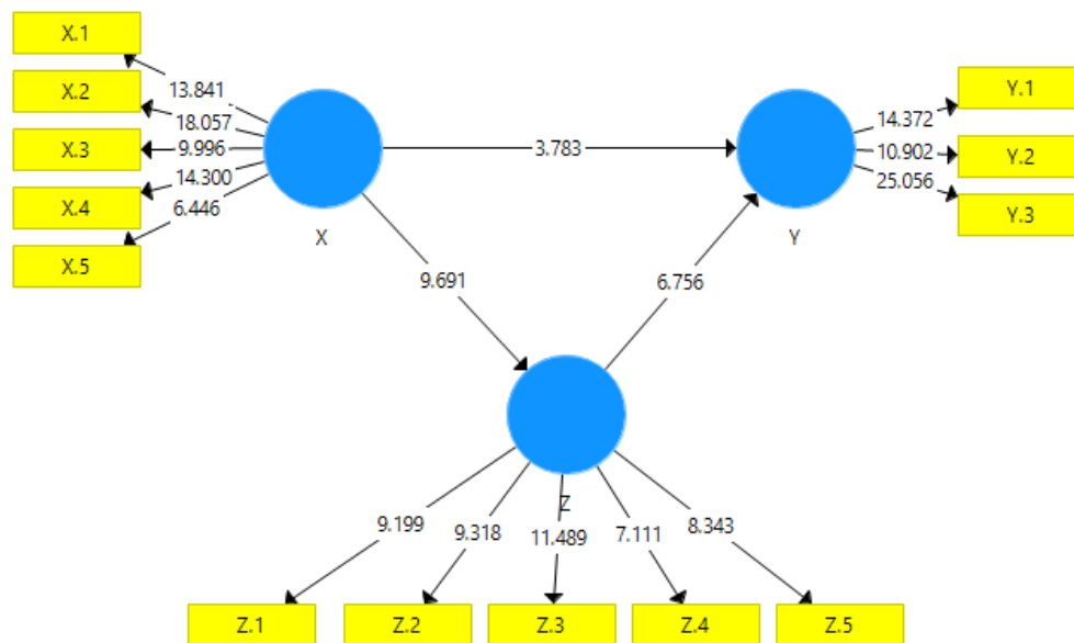
Gambar 4.1. Model PLS
